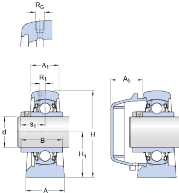
SYFWR 1.1/2 YZTHR Bearing 2D drawings and 3D CAD models
